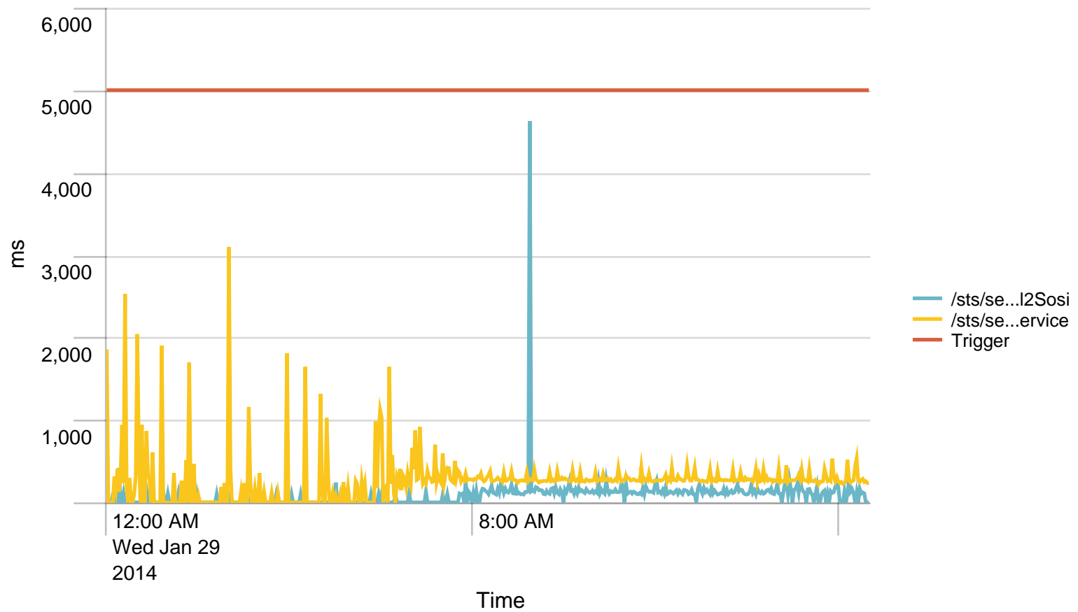
Average response time (ms) pr application / 1 minute - past day. Trigger: 5 sec
