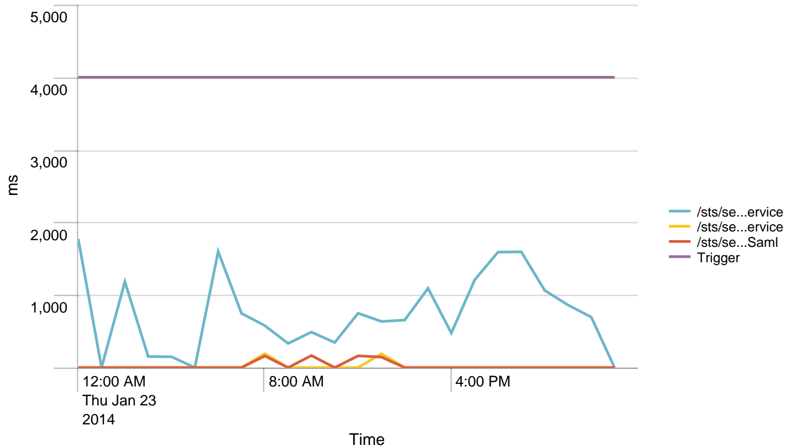
Average response time (ms) pr application / 1 hour - past day. Trigger: 4 sec
