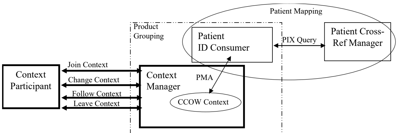
930 Figure D-1: Actor Grouping Diagram
